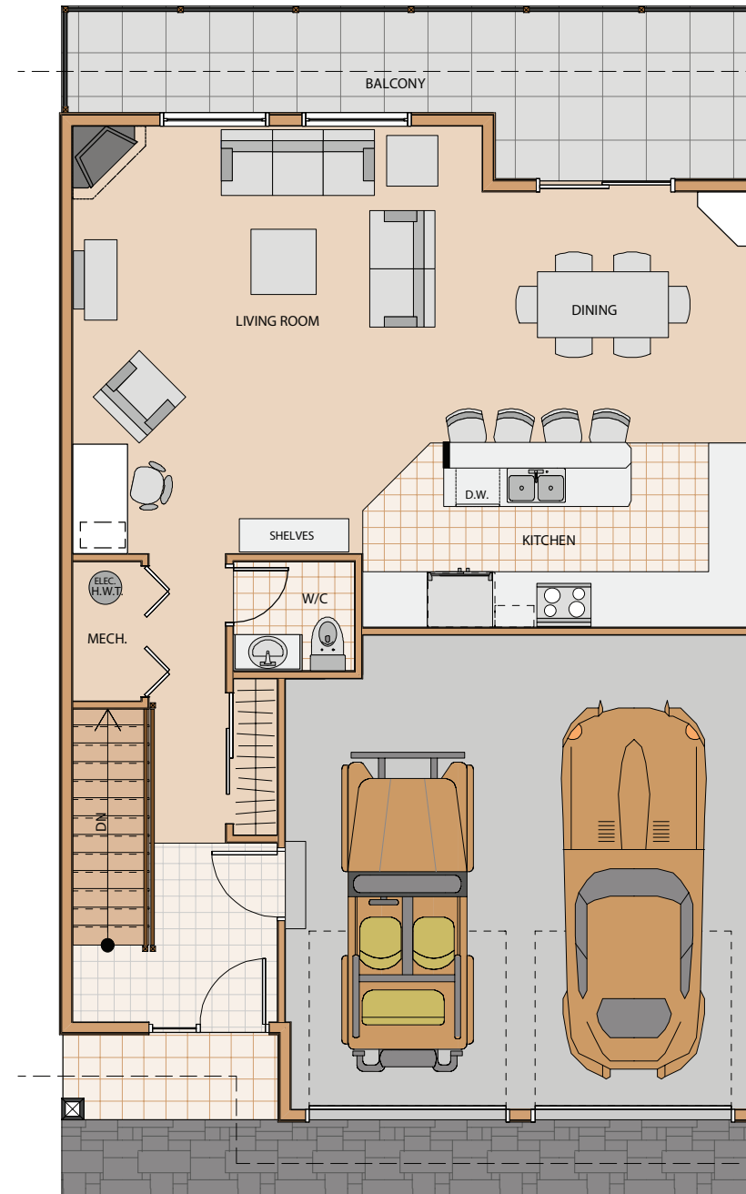
2 MAIN FLOOR PLAN Scale: 1/8" = 1'-0"
