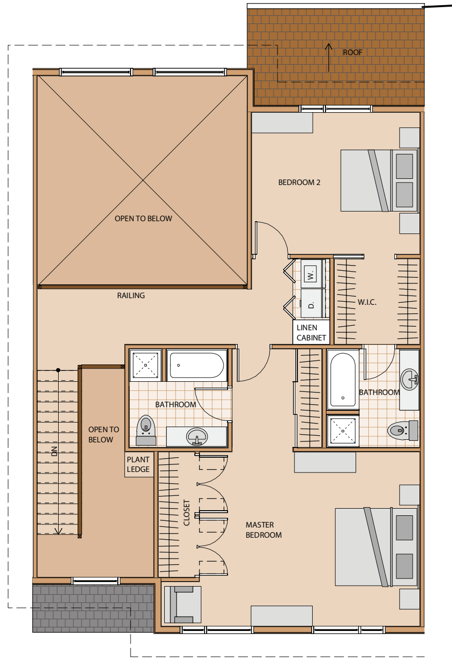
1 SECOND FLOOR PLAN Scale: 1/8" = 1'-0"
