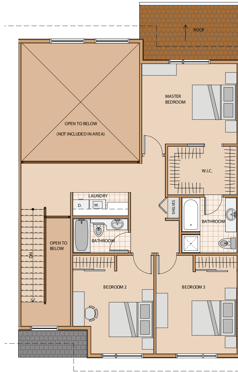
1 SECOND FLOOR PLAN Scale: 1/8" = 1'-0" 2nd Floor Area = 954.6 sq.ft.
